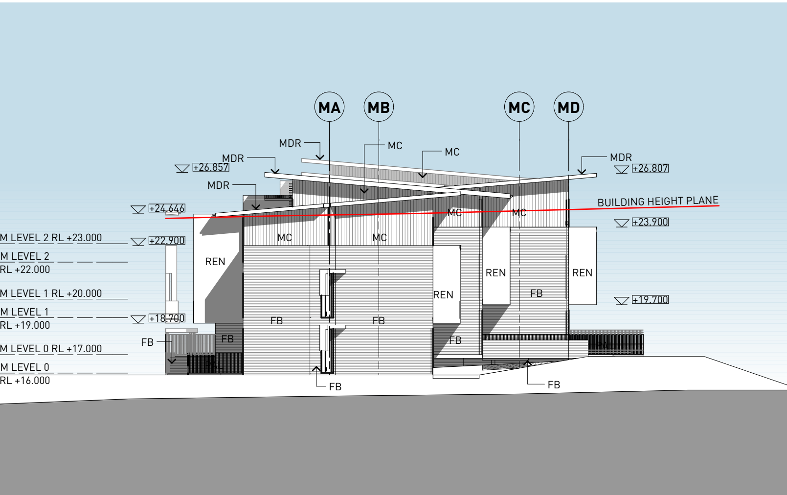
4 BUILDING M WEST ELEVATION 1:200
