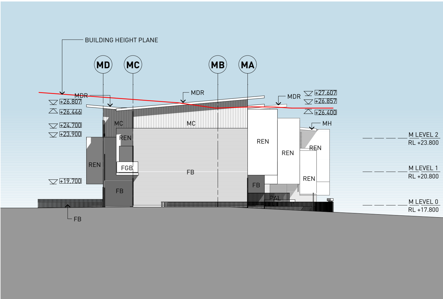
3 BUILDING M EAST ELEVATION 1:200
