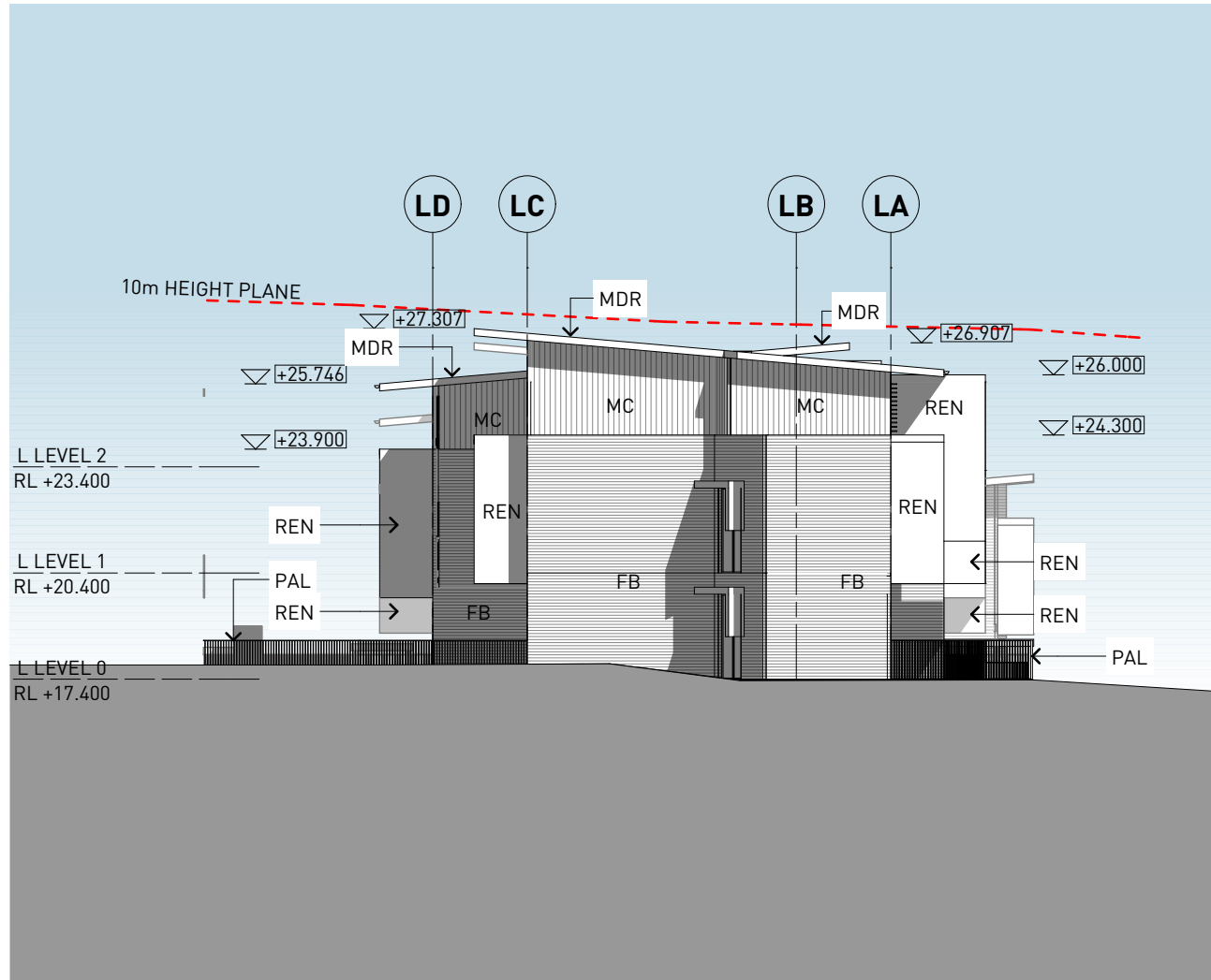
3 BUILDING L EAST ELEVATION 1:200
