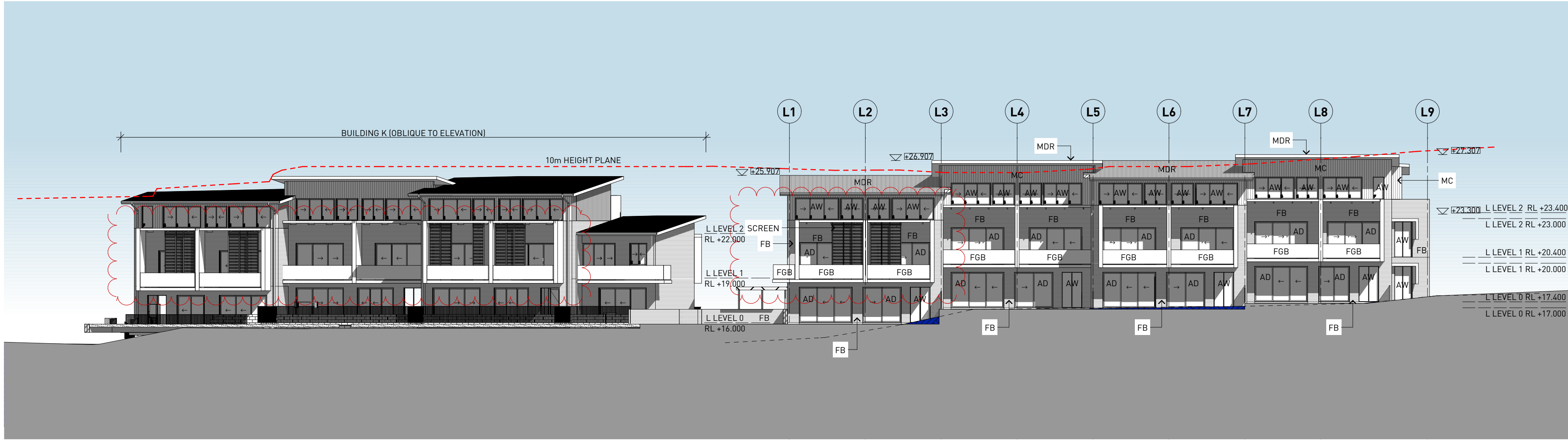
2 BUILDING L SOUTH ELEVATION 1:200
