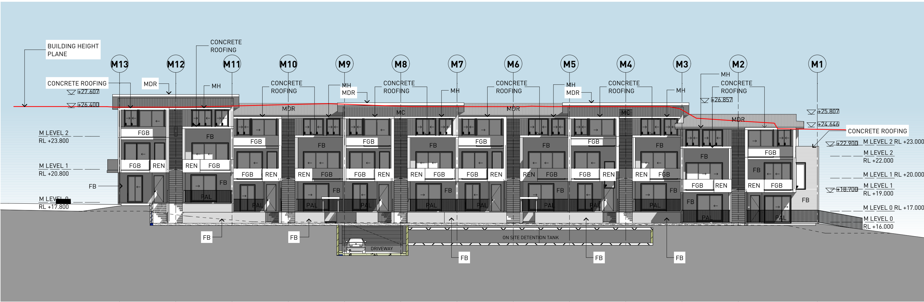
1 BUILDING M NORTH ELEVATION 1:200
