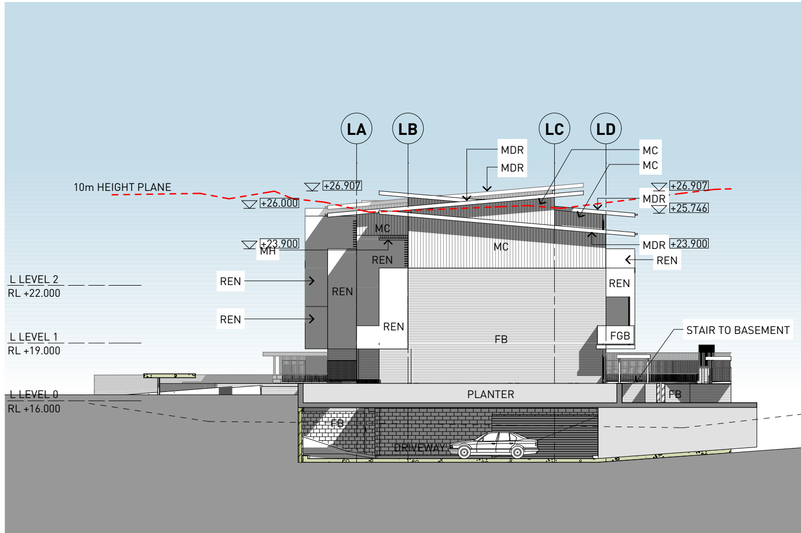
4 BUILDING L WEST ELEVATION 1:200
